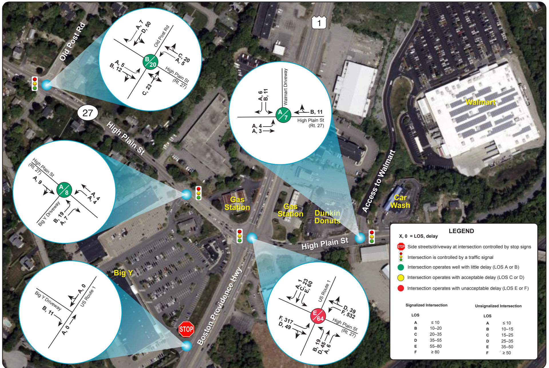
Figure 13 Walpole—Existing Conditions Weekday AM Peak-Hour LOS and Delays
