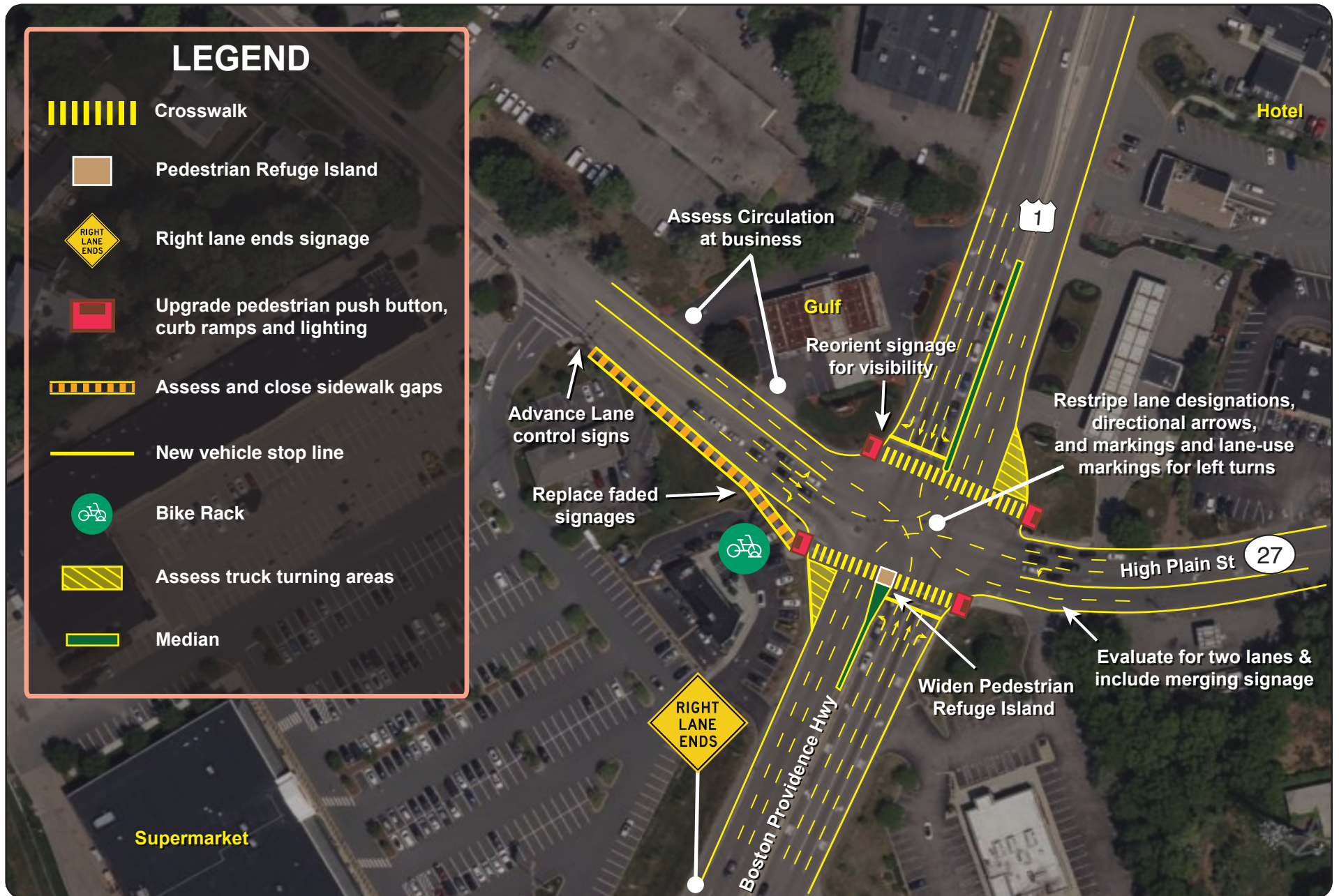
Figure 15 Walpole–Short & Long-Term Improvements US Route 1 at High Plain Street
