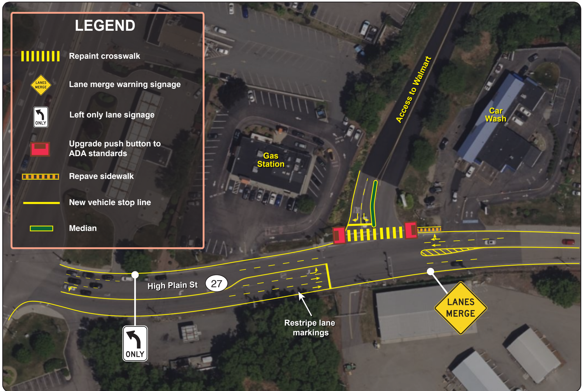
Figure 18 Walpole-Short & Long-Term Improvements Walmart Entrance at High Plain Street
