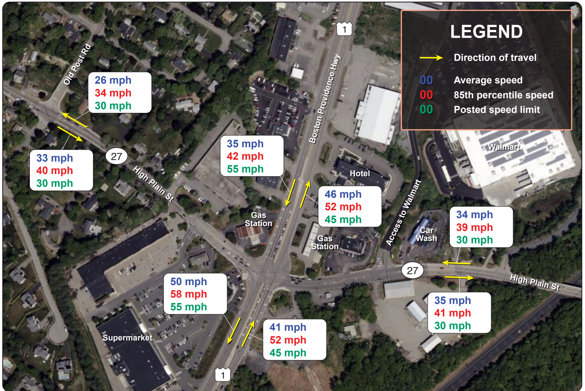
Figure 12 Walpole—Speed
