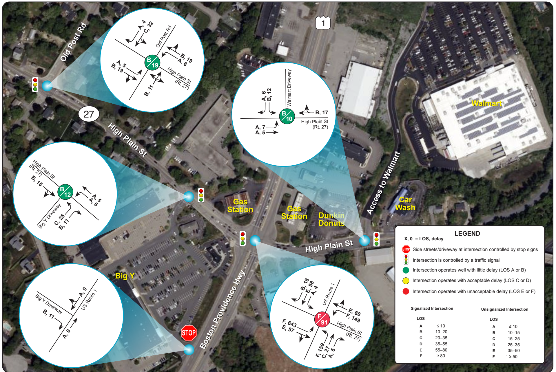
Figure 14 Walpole—Existing Conditions Weekday PM Peak-Hour LOS and Delays
